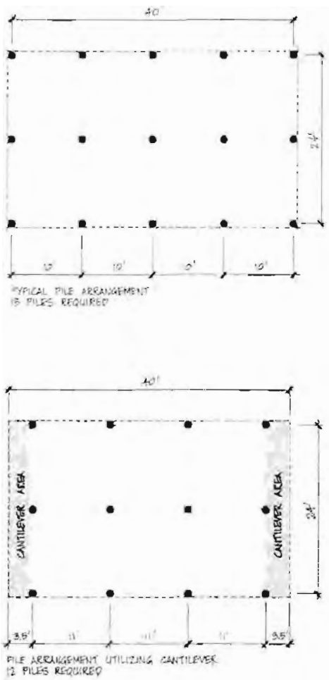
Figure 4.40. Cantilever Used to Reduce Number of Foundation Elements
