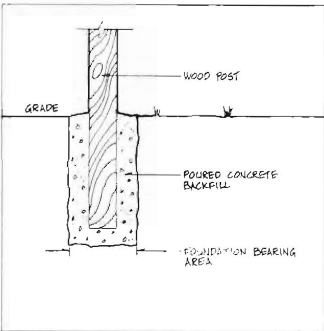
Figure 4.10. Concrete Backfill
