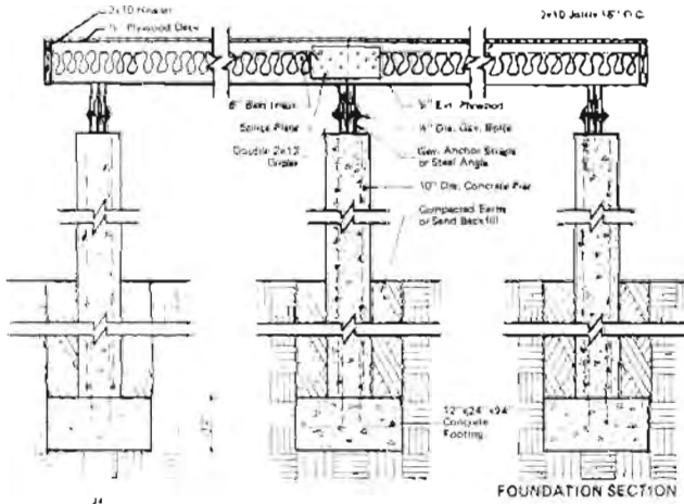
FOUNDATION SECTION
