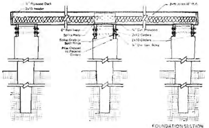
FOUNDATION SECTION
