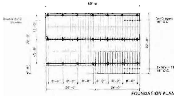
Figure 5.2. Elevated Foundations (Estimates are spring 1983.)
