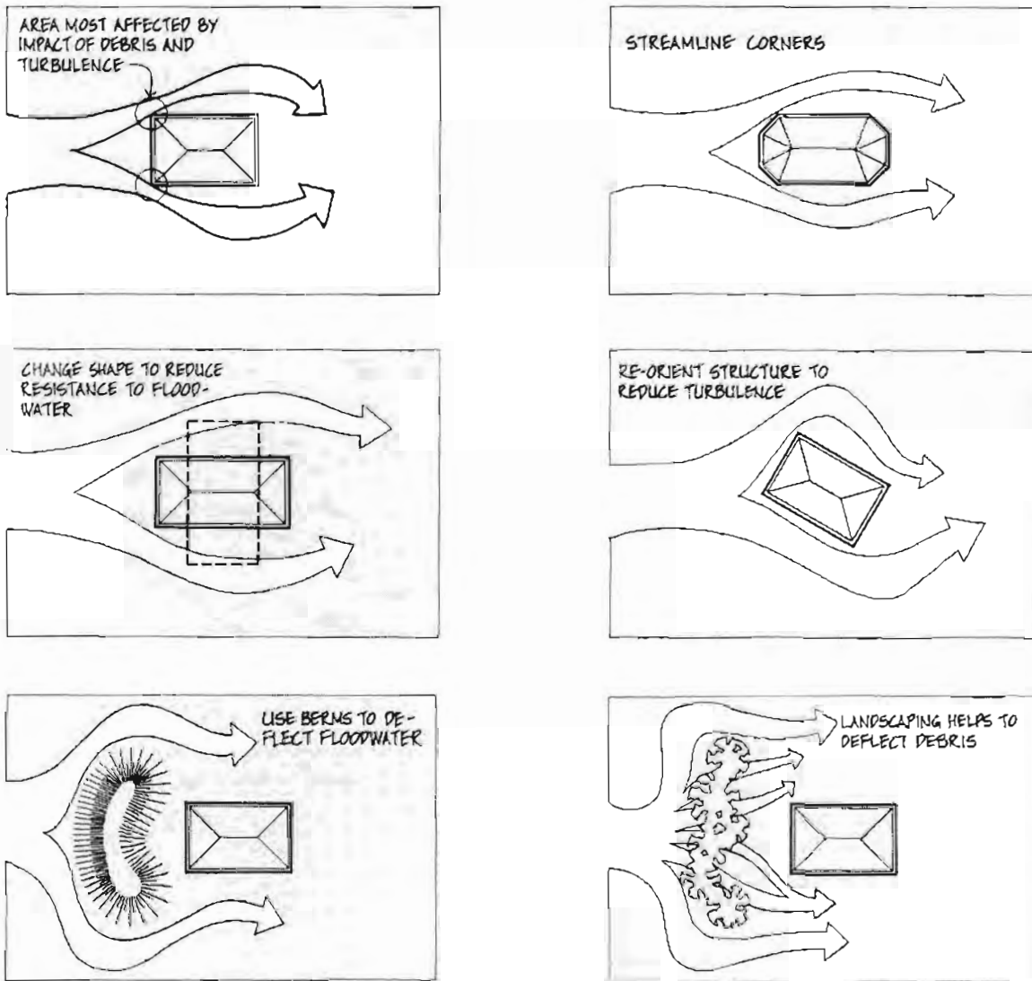
Figure 2.6. Site Design to Reduce Flood Hazards
