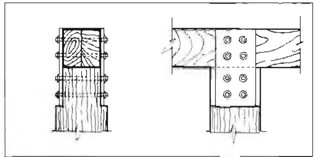
Figure 4.32. Dapped Gusset Plate Connection
