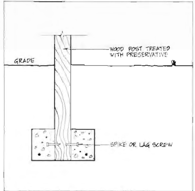
Figure 4.11. Spike Anchorage of Post
