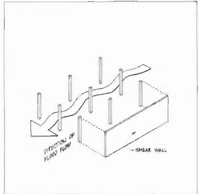
Figure 4.24. Shear Wall Bracing
