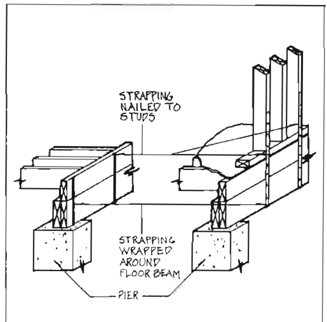
Figure 4.43. Metal Strapping
