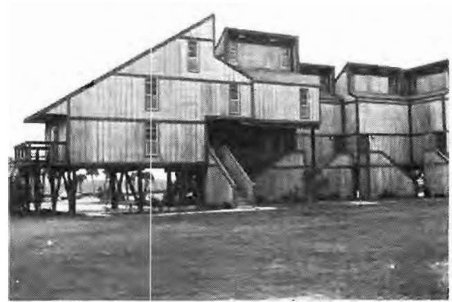
Figure 4.4. Elevation by Posts
