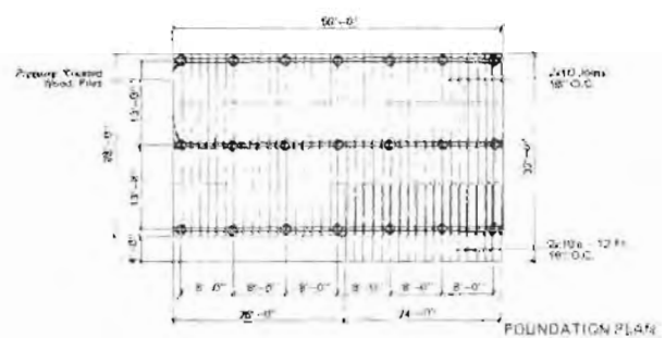
FOUNDATION PLAN
