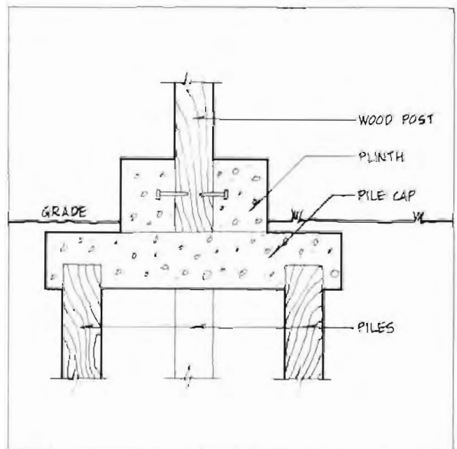
Figure 4.8. Post/Pile Foundation
