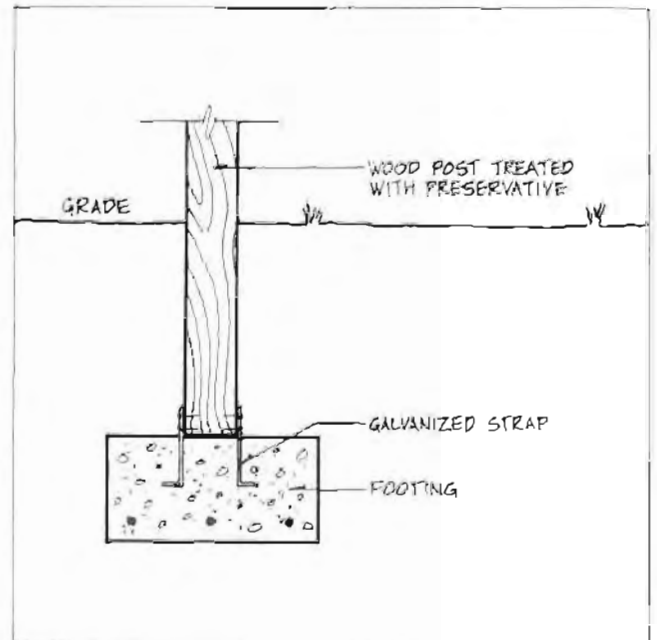
Figure 4.13. Galvanized Strap Anchorage Detail
