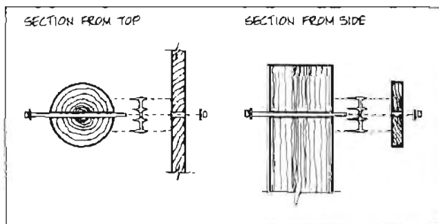
Figure 4.34. Spiked Grid
