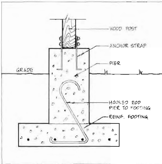
Figure 4.9. Post/Pier Foundation
