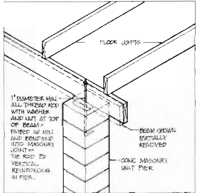
Figure 4.37. Masonry Pier - Bolt Through Beam
