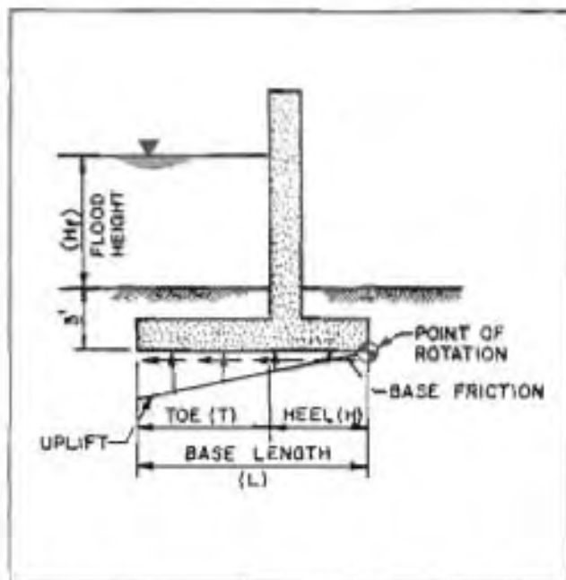
Figure III-50. Stability-Cantilever Floodwalls
