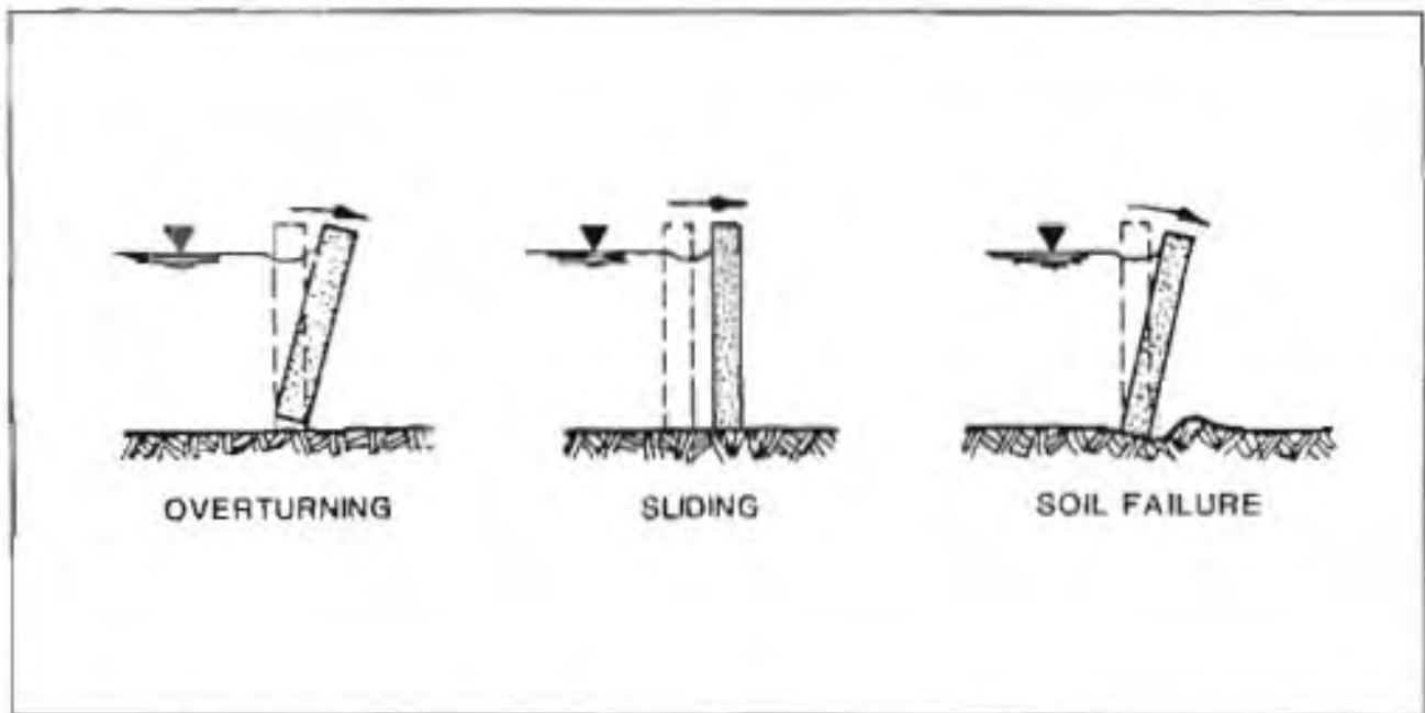
Figure III-48. Floodwall Stability
