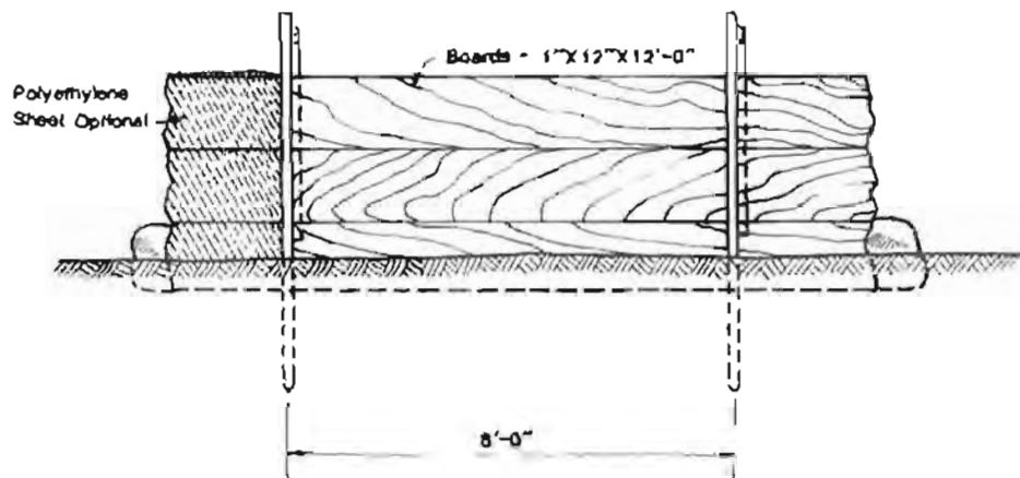
RIVERSIDE ELEVATION
