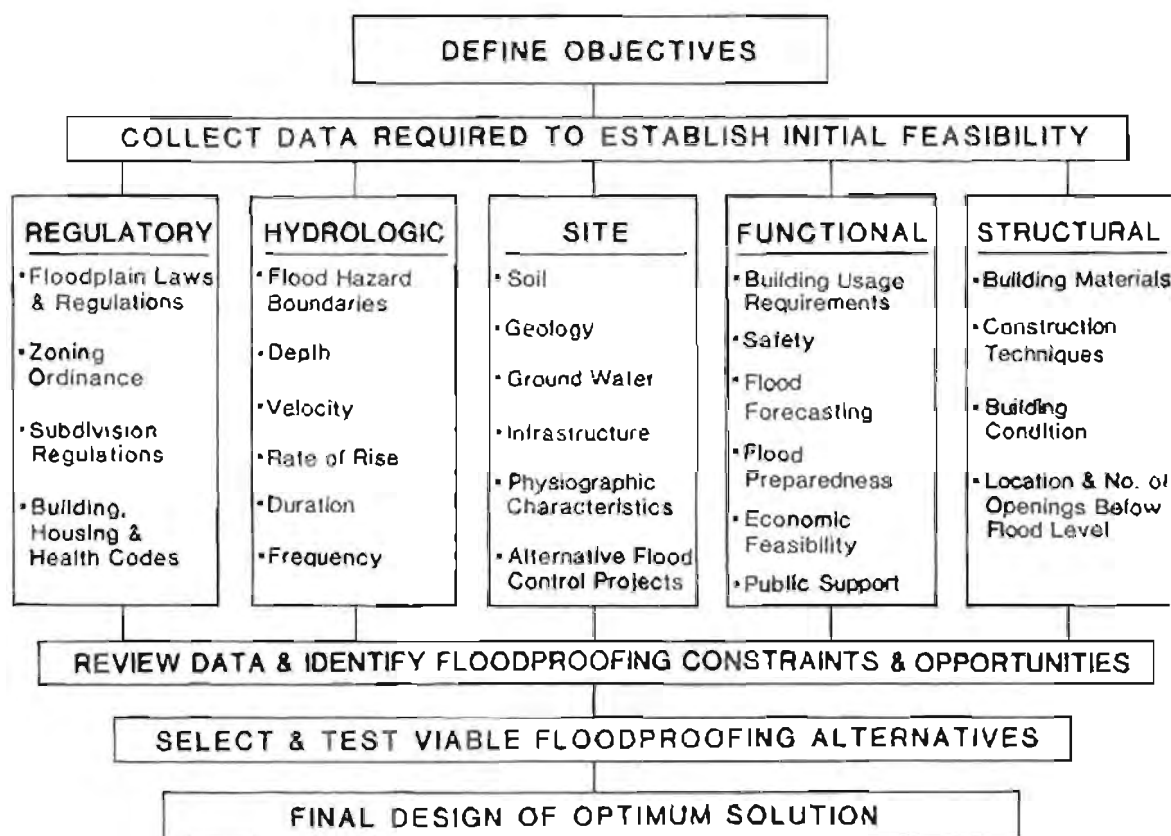
Figure II-1. General Floodproofing Design Process
