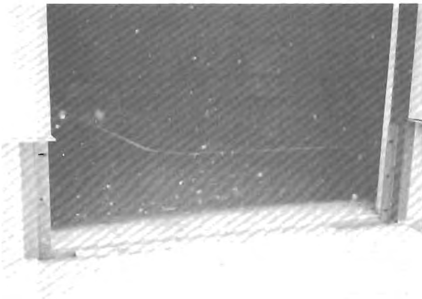
Frame for mounting flood shield on loading dock door. A 4" x 4" piece of timber is used to facilitate traffic over a slot designed to receive and seal the flood shield.
