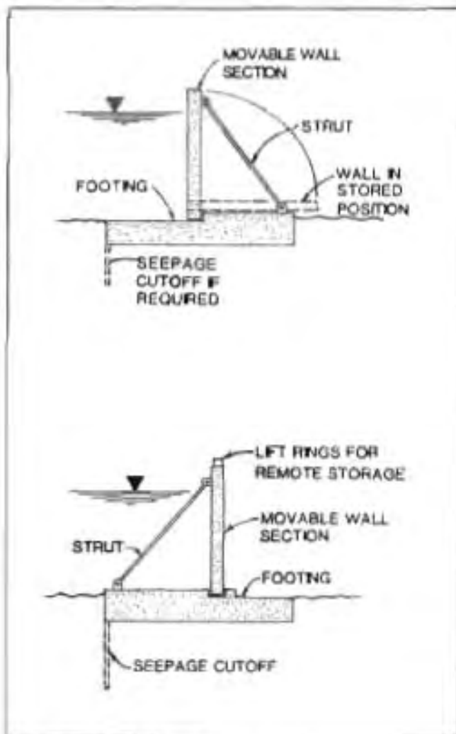
Figure III-52. Movable Floodwalls
