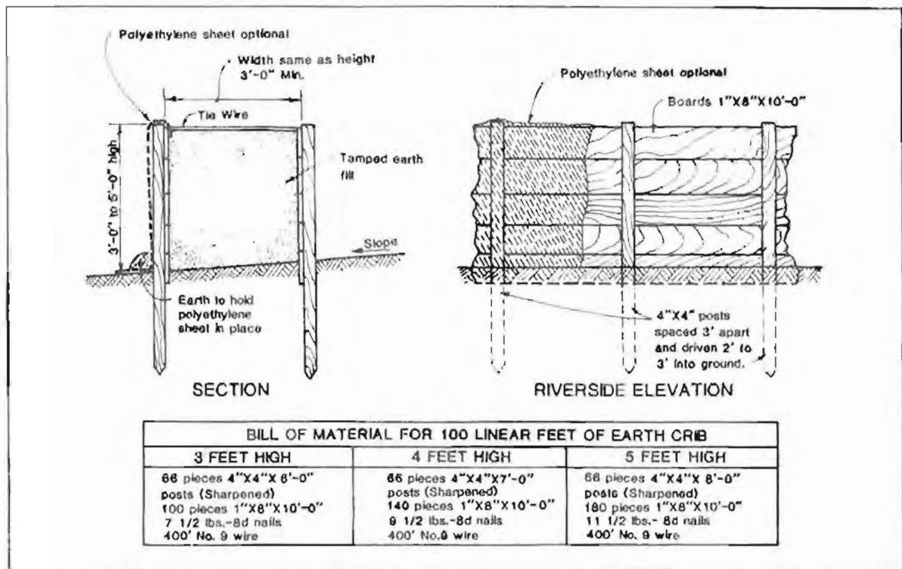
Figure IV-3. Earthfill Crib Retaining Wall
