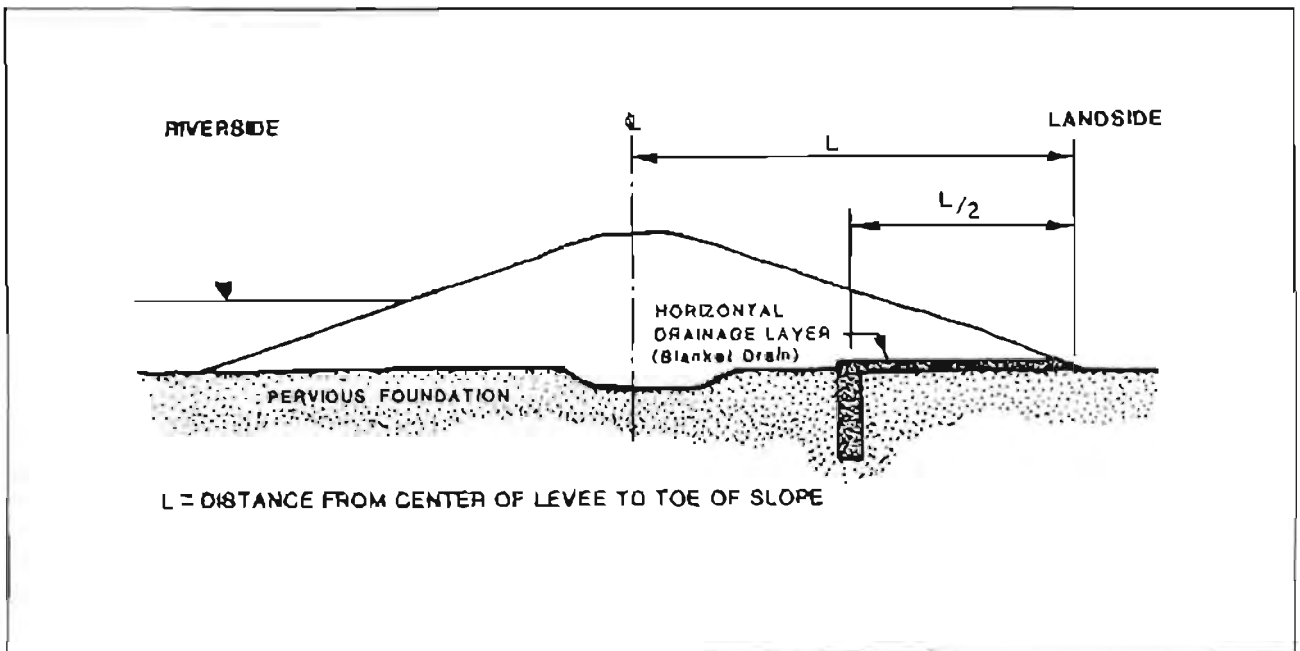
Figure III-45. Blanket Drain Beneath Levee
