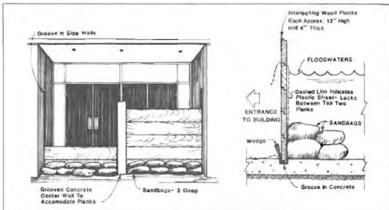
Figure IV-5. Typical Stop Log Barrier
