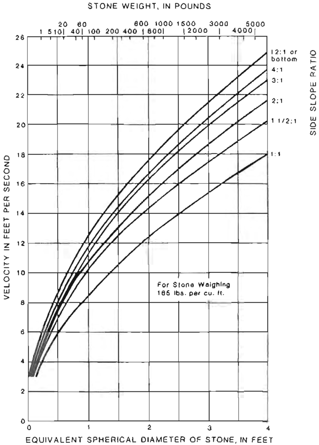
Figure III-56. Size of Stone That Will Resist Displacement for Various Velocities and Side Slopes Source: Adapted from Subcommittee Report on Slope Protection, American Society of Civil Engineers Proceedings, June, 1948
