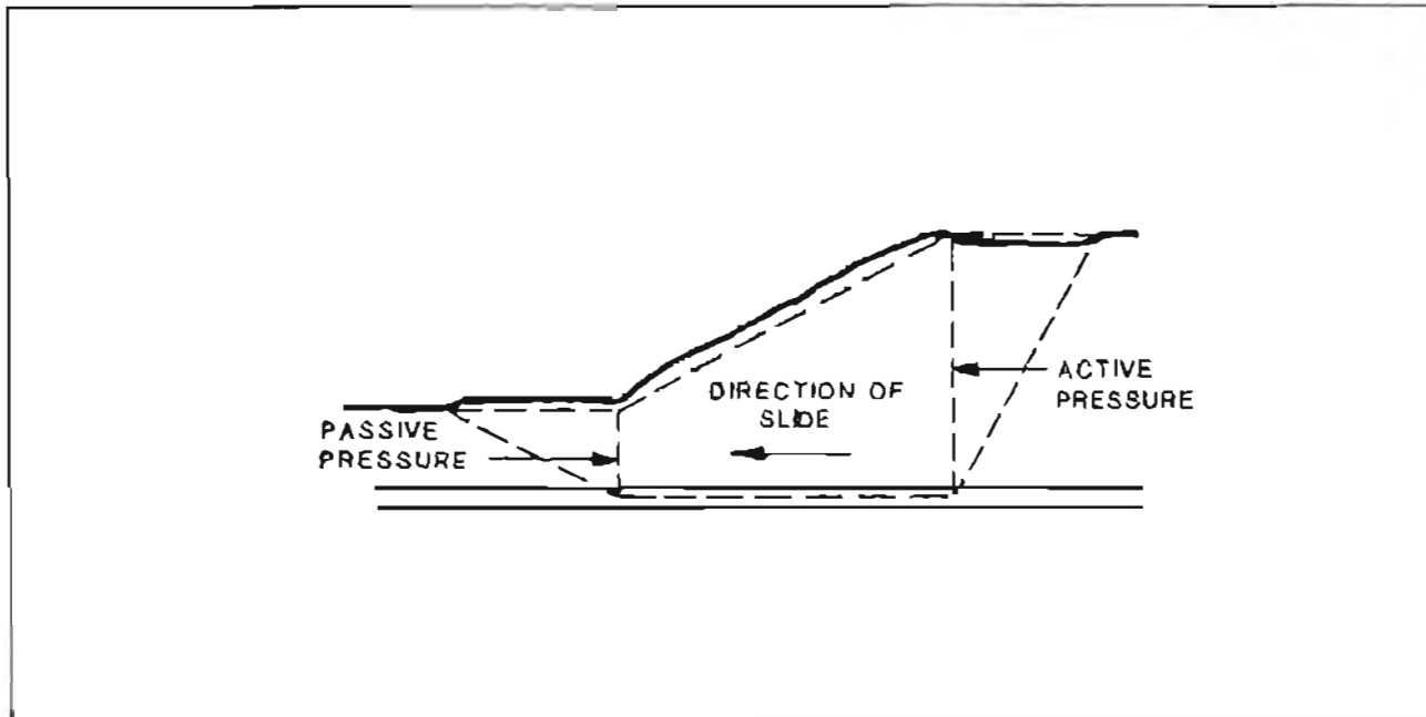
Figure III-54. Translatory Slide
