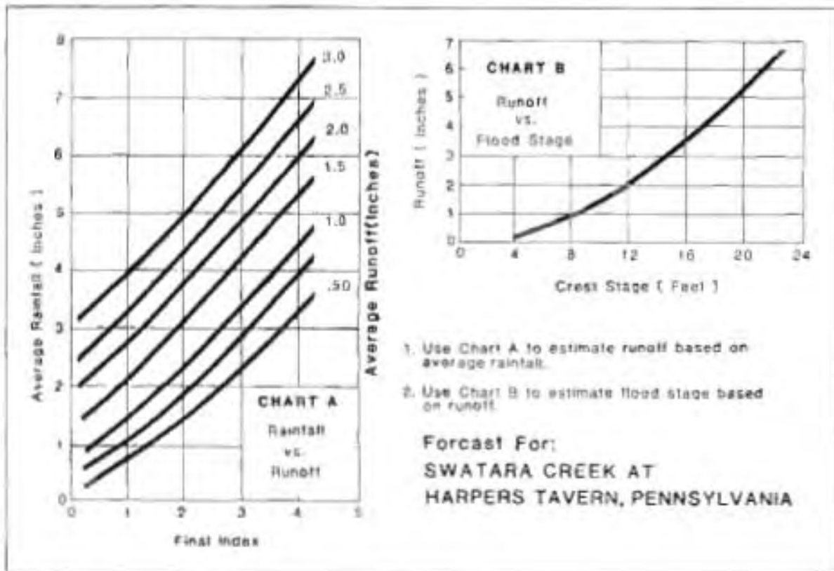
Figure II-9. Flood Forecasting Charts
