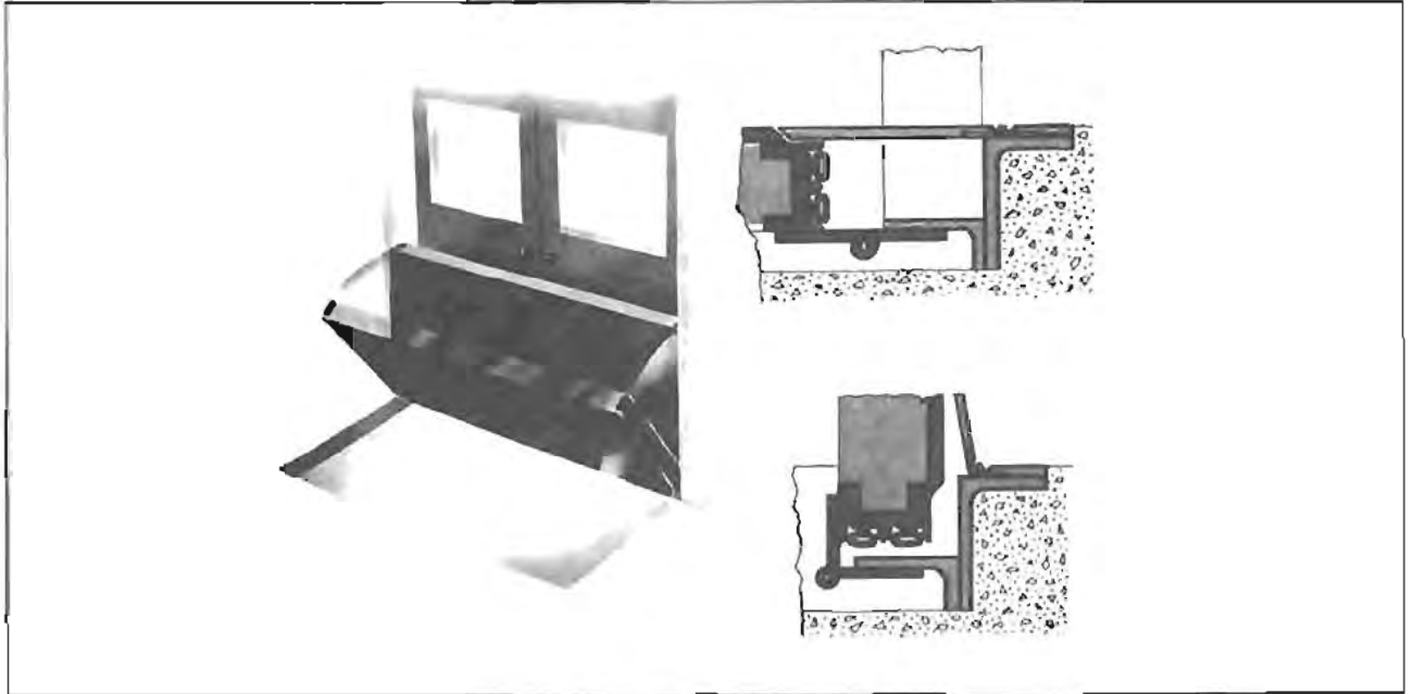
Figure III-35. Bottom Hinged Flood Barrier
