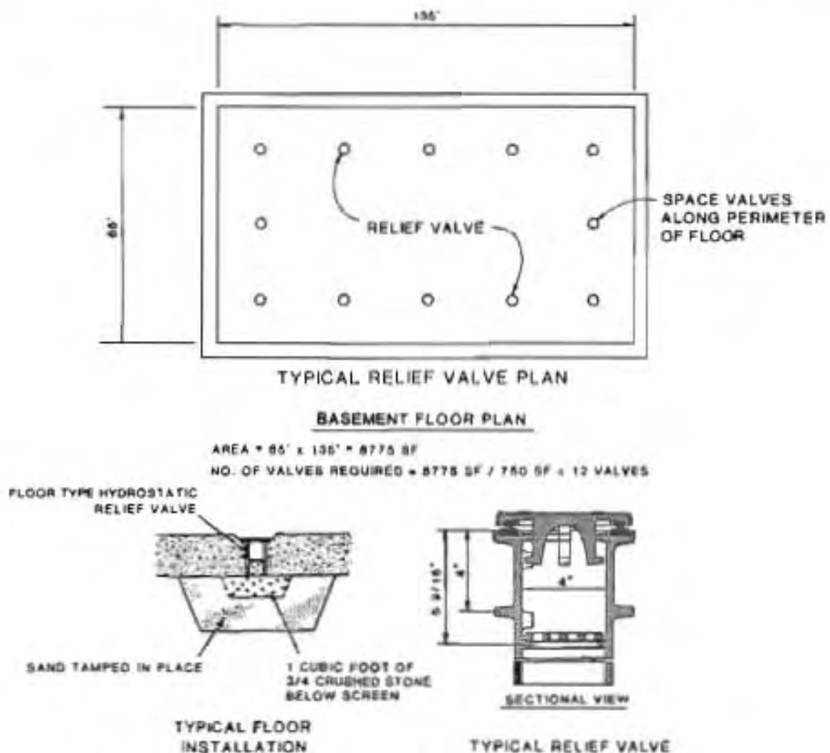
Figure III-20. Typical Pressure Relief Valve System
