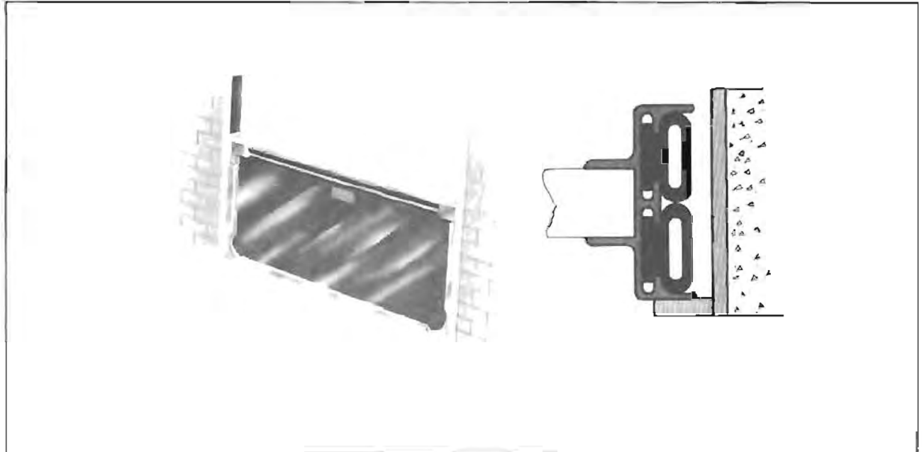
Figure III-36. Manually Installed Flood Barrier
