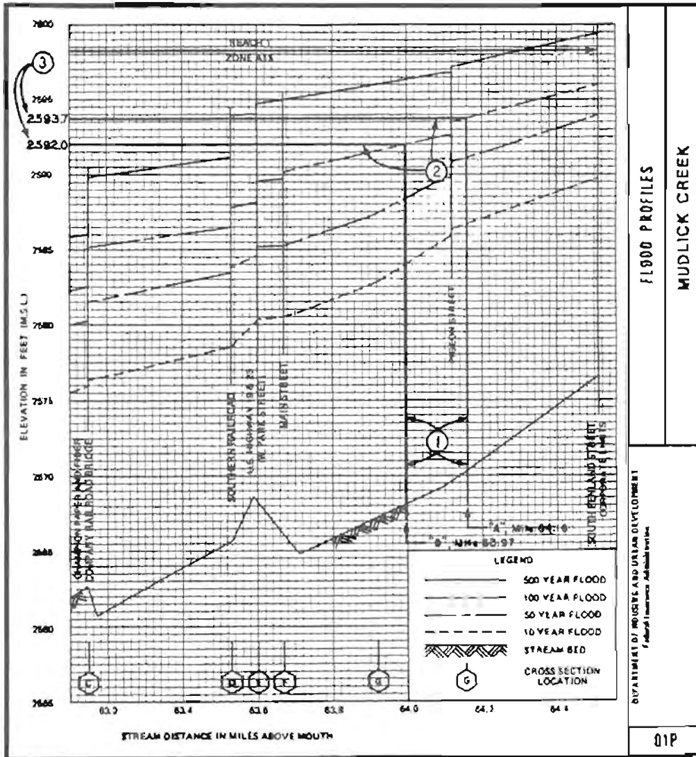
FIGURE F-2 EXAMPLE FLOOD PROFILE
