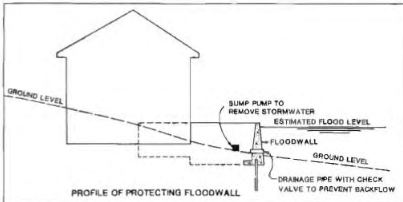
Figure 1-6. Flood Protection With Low Floodwall
