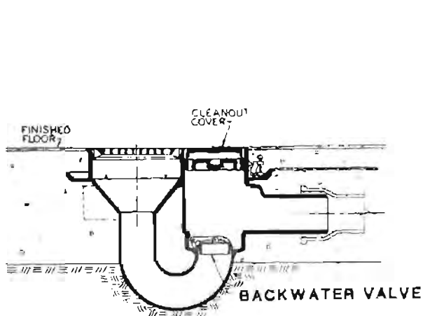
VARIOUS EXAMPLES OF BACKWATER VALVES
