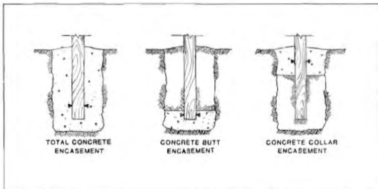
Figure III-1. Concrete Backfill
