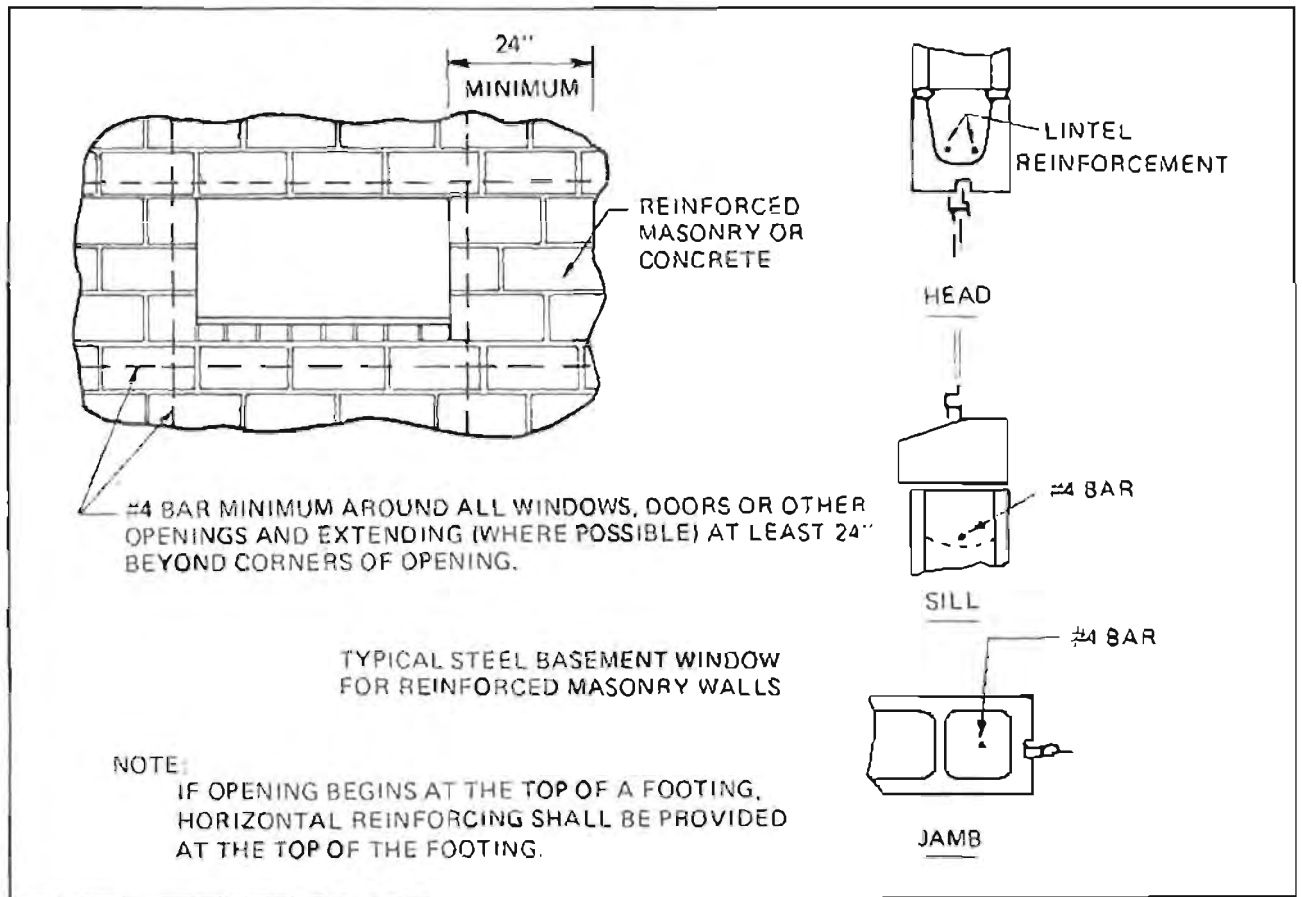
Figure III-25. Recommended Reinforcement of Masonry Walls Around Small Openings
