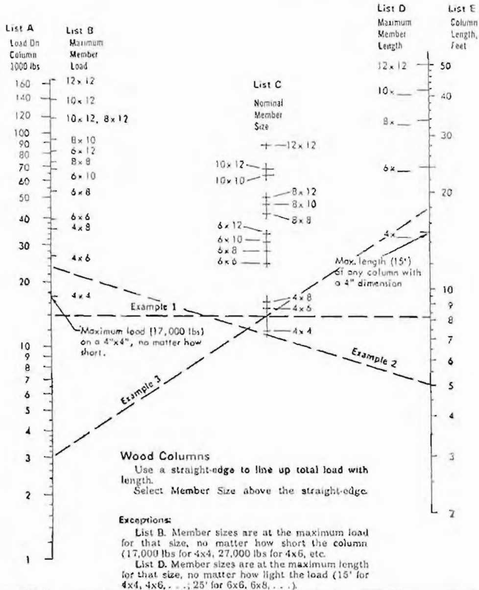
Figure III-6. Approximate Loads on Wood Posts
