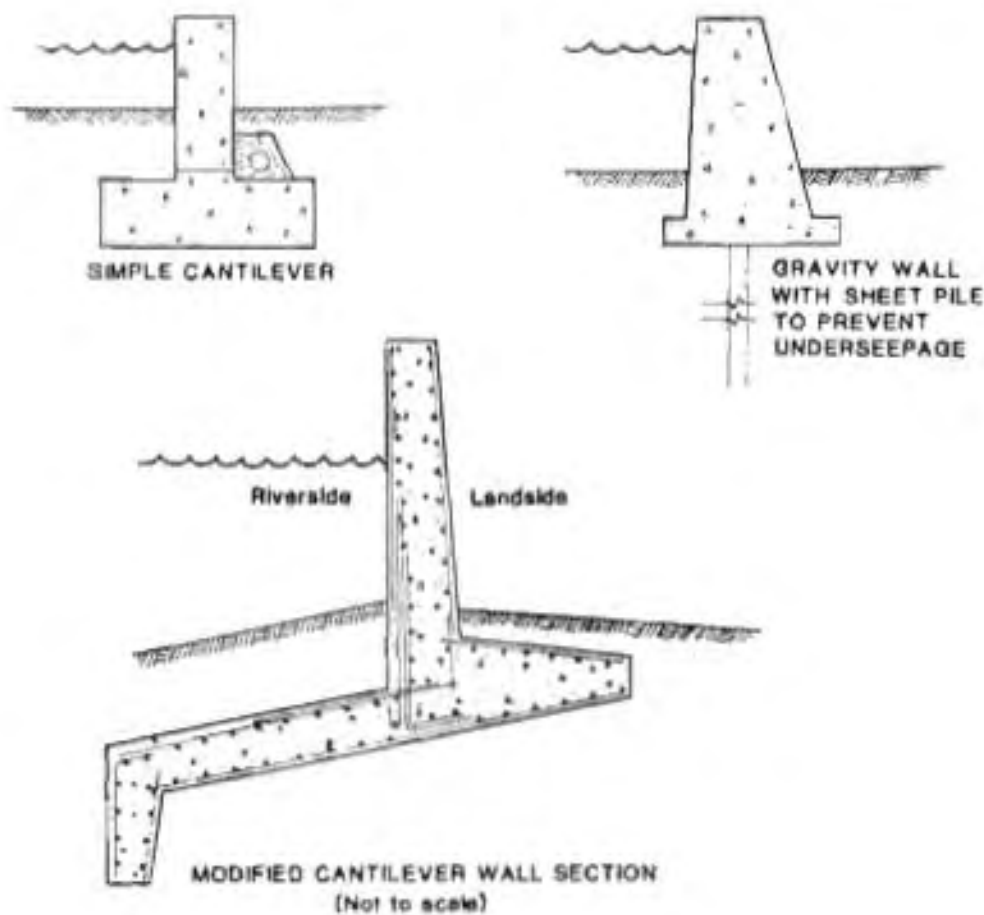
Figure 1-3. Typical Floodwall Configurations
