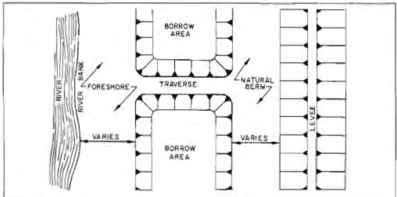
Figure III-55. Typical Levee and Borrow Areas
