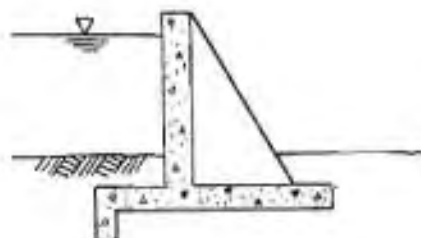
BUTTRESS
