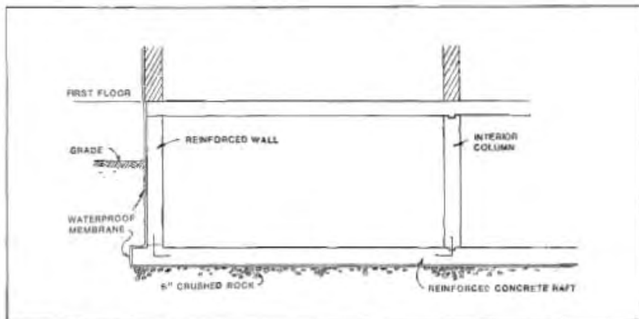
Figure III-16. Raft or Mat Foundation
