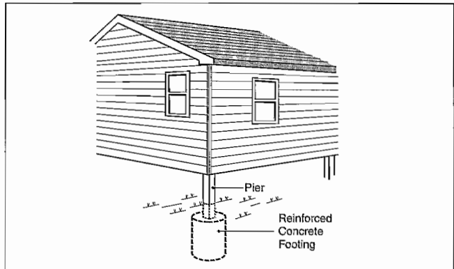
While commonly used in riverine areas, piers are not suitable to withstand the hydrodynamic forces associated with coastal flooding.
